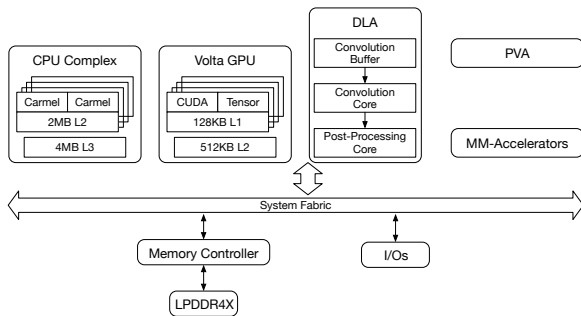
Figure 4: The NVIDIA Jetson AGX Xavier Architecture
